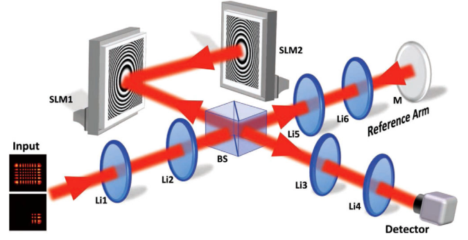
FIG. 3. Schematic of the optical setup. For the noninterferometric measurement, only the arm of the Michelson interferometer that contains the SLMs is used. The anisotropic lenses L1 and L3 are implemented on SLM1, while L2 is implemented on SLM2. The input field is imaged onto SLM1 using a 4f system (unit magnification) formed by lenses L1 and L2 . In the reference arm (used for the interferometric measurements), the field is relayed onto mirror M using another telescope formed by lenses L5 and L6 (magnification = 0.5). The interference signal is relayed to the CCD detector using the 4f system formed by lenses L3 and L4 (magnification = 0.5). Distances are not drawn to scale.
