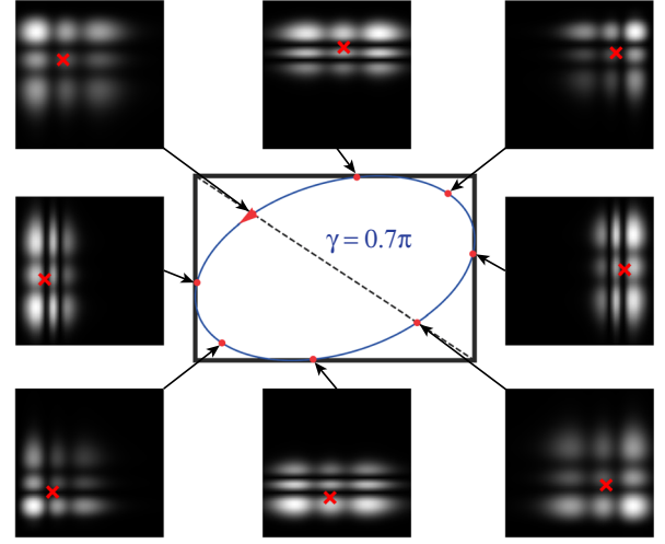
FIG. 5. Evolution of the intensity distribution of a blocked HG beam as the Gouy phase varies, and the corresponding elliptic trajectory traced by the centroid for a fixed PB phase.
