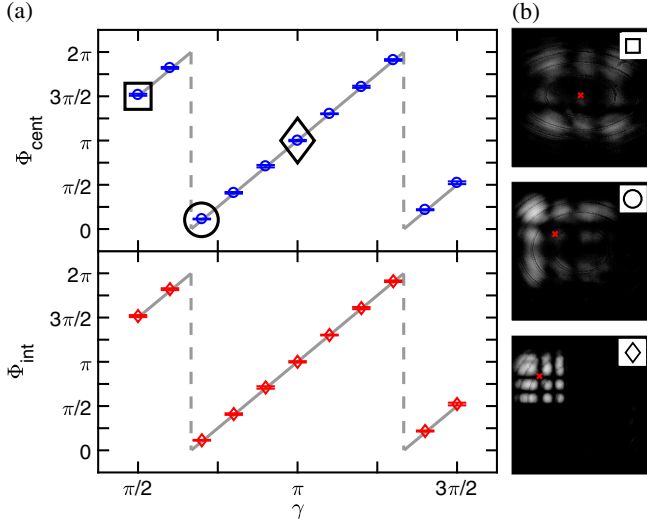
FIG. 4. PB phase measurement results. (a) Measured PB phase as a function of \gamma using the centroid of the blocked beam (circles, top panel) and interferometric measurements (diamonds, bottom panel). The noninterferometric results are wrapped onto [0, 2\pi) for comparison with the interferometric ones. Error bars are shown for both, as well as the theoretical value (gray line). (b) Measured intensity of the transformed blocked beam (plotted on a log scale) with centroids as red crosses, for different \gamma . The symbols at the insets correspond to the markers in (a).
